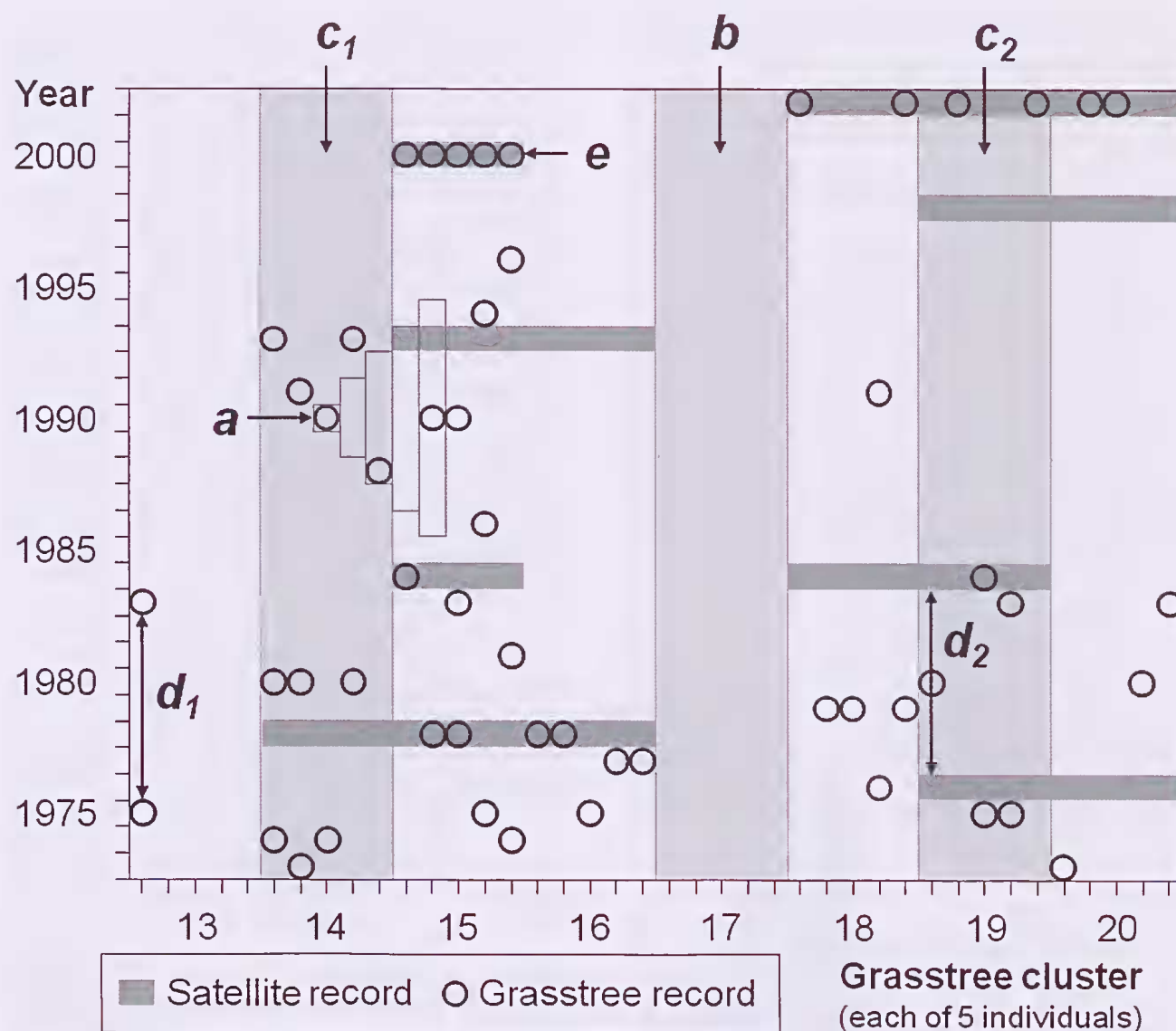
Figure 2 A comparison of grasstree and satellite records for 8 (of 20) analysed grasstree clusters, illustrating elements of the data and analysis. (a) The five precision windows employed by Miller et al. (2007) illustrated here for 1990 with (from left): a 1 year window (i.e. 'exact' precision) with a false positive grasstree record (a grasstree fire not matched by a satellite fire within the window); 3 year (i.e. \pm 1 years) and 5 year windows ( \pm 2 years), both true negatives (no grasstree fire in 1990 + no satellite fire in the window); a 7 year window ( \pm 3 years) showing a false negative (no grasstree fire but a positive satellite record within the window not otherwise matched by a closer grasstree fire); and a 9 year window ( \pm 4 years)—a true positive (a grasstree fire + an otherwise unmatched positive satellite record in the window). (b) The cluster of five grasstrees mistakenly omitted from Miller et al. (2007) figure 2. (c) Clusters of five grasstrees with contrasting ratios of grasstree:satellite fire incidence: c_1 with 11 v 5, and c_2 with 7 v 20. (d) A pair of matching 8 year inter-fire periods: the first of three in the grasstree record ( d_1 ), and the first of five in the satellite record ( d_2 ). (e) The only example of spatial aggregation (i.e. among individual grasstrees in a cluster) in positive agreement between the satellite and grasstree records.
